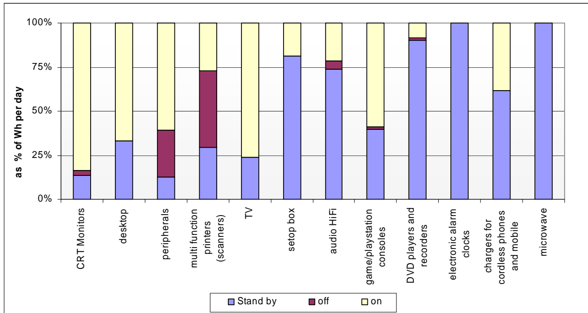
Figure 5. Stand by, off and on mode electricity consumption as % of their total consumption [ISR-UC]
