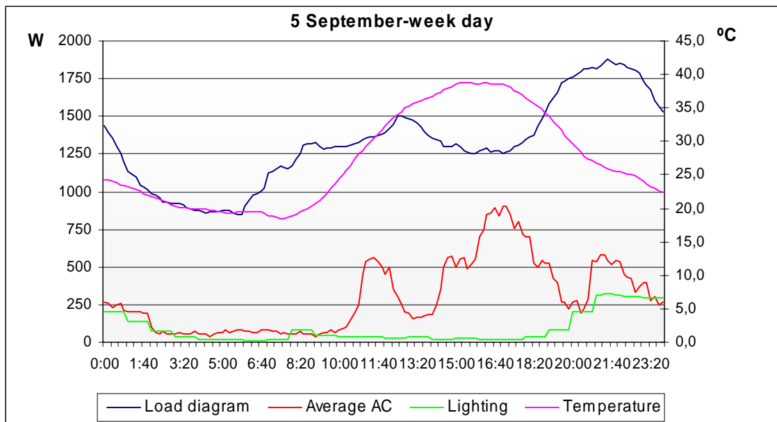
Figure 7. Daily Load profile of air conditioning and lighting in a normal working day [ISR-UC]
