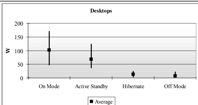
Figure 3a .Power consumption of desktop PCs, for each operating mode [ISR-UC, 2006]
