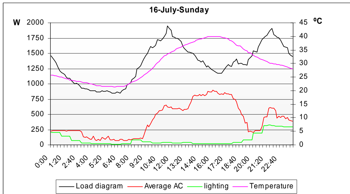
Figure 6. Daily Load profile of air conditioning and lighting in a weekend day [ISR-UC]
