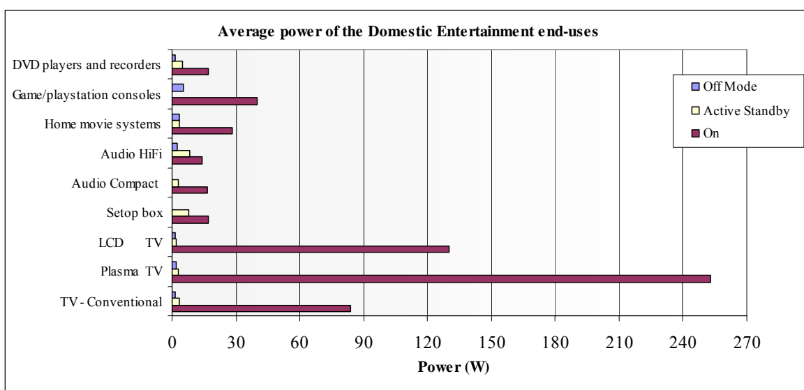
Figure 4. Average power of domestic entertainment loads in the distinct operating modes [ISR-UC, 2006]
