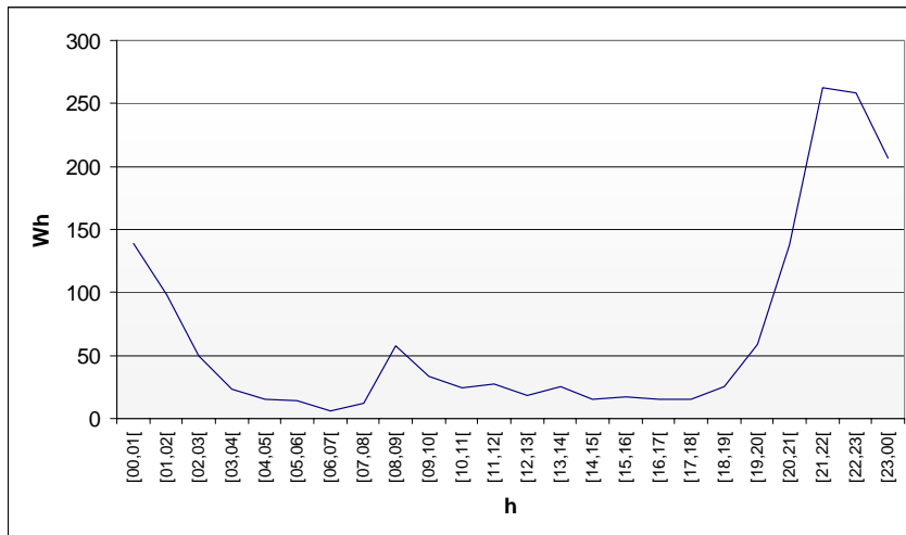
Figure 13. Average daily lighting load diagram [ISR-UC, 2006]
